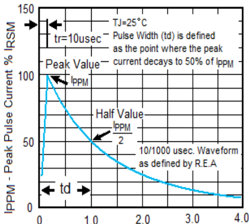
Fig. 3 Pulse Waveform
