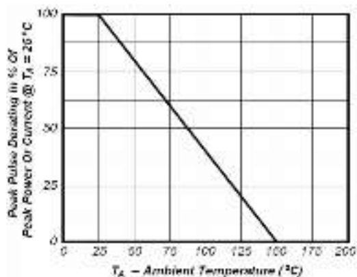
Fig1. Pulse Dearting Curve
