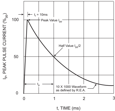
Fig. 1 Pulse Waveform
